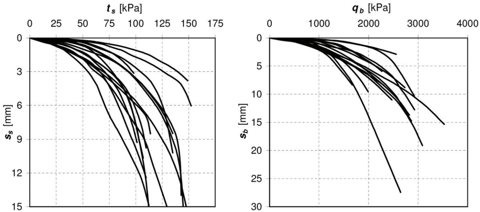
Fig. 3. Graphs of unit resistances t_s and q_b
