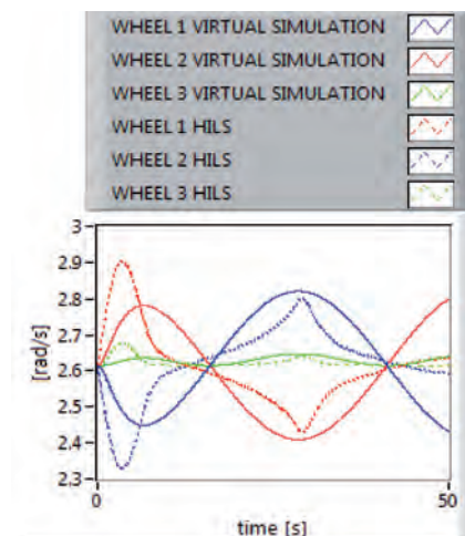
Fig. 11. Wheel speeds (HILS)
