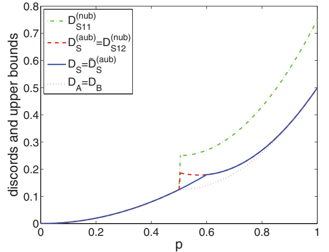
FIG. 2. (Color online) Geometric discords and their tight upper bounds for the state \rho(p, \phi = \pi/2) , given by Eq. (46), as a function of the parameter p : The CC discord, D_S [solid (blue) curve], and CQ and QC discords, D_A = D_B [dotted (magenta) curve], together with the adaptive upper bound, D_S^{(\text{aub})} [dashed (red) curve], and unoptimized nonadaptive upper bounds, D_{S11}^{(\text{nub})} = D_{S22}^{(\text{nub})} [dot-dashed (green) curve]. We note that the optimized upper bound \tilde{D}_S^{(\text{aub})} = D_S and D_S^{(\text{aub})} = \tilde{D}_{S12}^{(\text{aub})} = \tilde{D}_{S21}^{(\text{aub})} for any p . All the upper bounds, except \tilde{D}_S^{(\text{aub})} , are discontinuous at p = 1/2 , while the corresponding vertical lines are added for clarity only.
