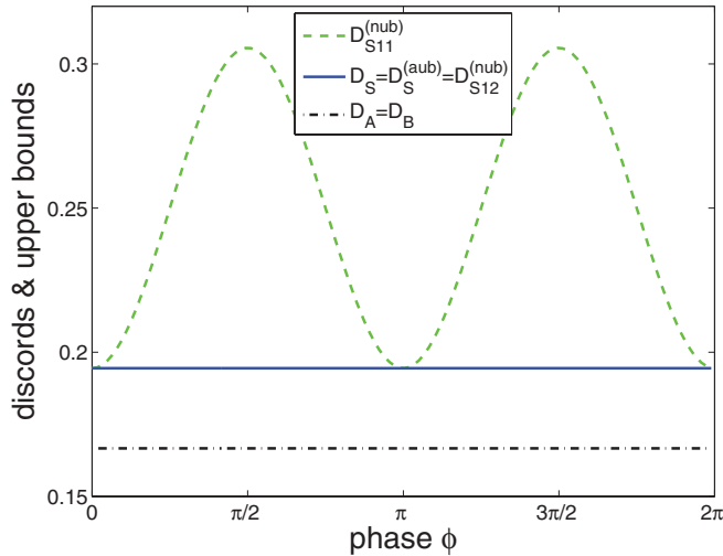
FIG. 3. (Color online) Same as Fig. 2, but for the state \rho(p, \phi) as a function of phase \phi for fixed p = 2/3 .
