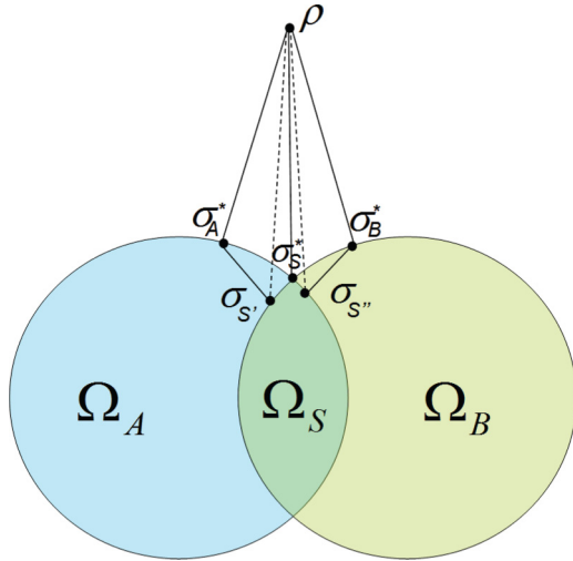
FIG. 1. (Color online) Venn-type diagram showing the sets of the CC ( \Omega_S = \Omega_{AB} ), CQ ( \Omega_A ), and QC ( \Omega_B ) states together with the closest states \sigma_i^* ( i = S, A, B ) according to the CC ( D_S ), CQ ( D_A ), and QC ( D_B ) geometric discords, respectively. States \sigma_{S'} and \sigma_{S''} , which correspond to the adaptive upper bound D_S^{(aub)} , are the closest CC states for \sigma_A^* and \sigma_B^* , respectively. This is an intuitive graph, but more precisely, the point \sigma_A^* ( \sigma_B^* ) should be on the line between \rho and \sigma_{S'} ( \sigma_{S''} ).
