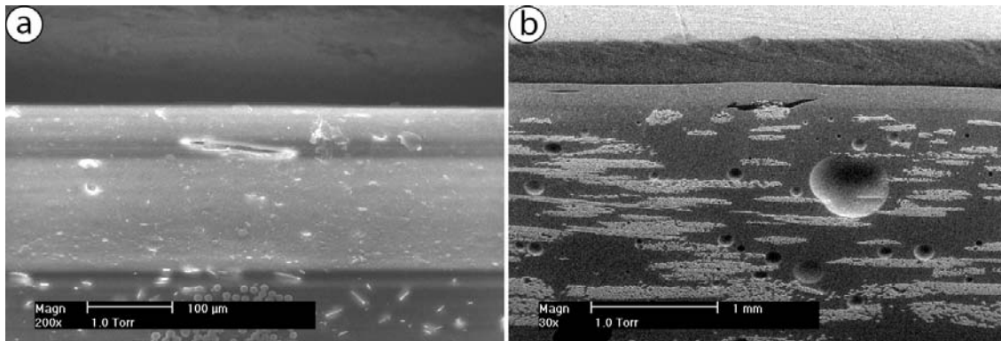
Fig. 3. Damage corresponding to 0% and 10% nanoparticles after 1000 hours exposure in water at 37°C
