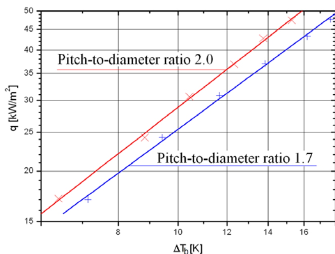
Fig. 6. Influence of pitch-to-diameter ratio for water boiling at atmospheric pressure; pitch-to-diameter ratio: + 1.7, x - 2.0
