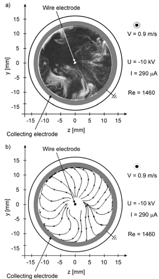
Figure 7. Instantaneous image of the dust particles (a) and averaged flow streamlines (b) in the circular ESP. Average total discharge current 290 \mu\text{A} . Negative voltage 10 kV. \odot - shows the direction of the primary flow.
