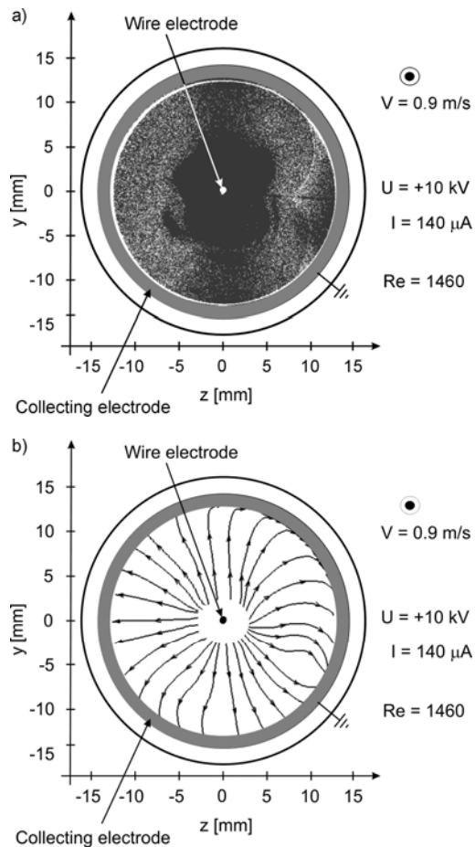
Figure 6. Instantaneous image of the dust particles (a) and averaged flow streamlines (b) in the circular ESP. Average total discharge current 140 \mu\text{A} . Positive voltage 10 kV. \odot - shows the direction of the primary flow.
