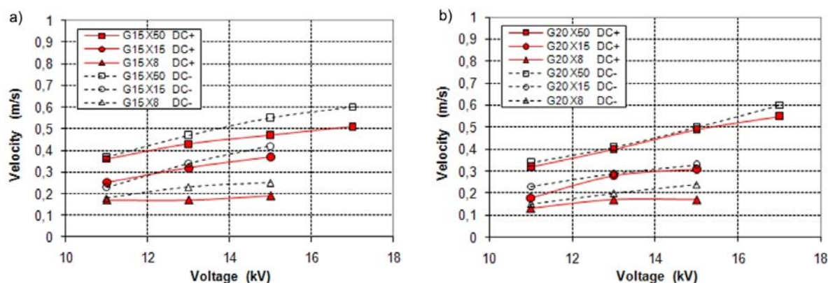
Figure 28. The flow average velocity induced in the self-pumped ESP for (a) G = 15 and (b) G = 20 as a function of the applied voltage
