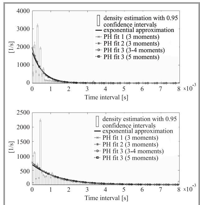
Fig. 6. Histograms of message inter-departure times at the P-CSCF (top, c^2 = 2.16 ) and S-CSCF (bottom, c^2 = 1.36 ) CPU_o (data set 1, \lambda_{INV} = 100 [1/s]).
