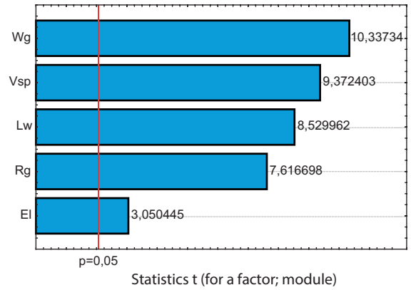
Fig. 2. Standardised effects Pareto chart (model I)
