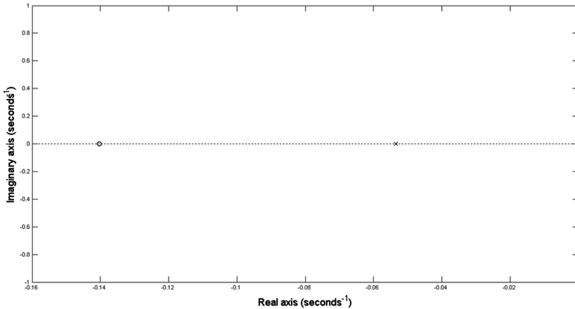
Figure 5. Plant pole-zero map.
