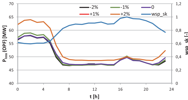
Fig. 3. Power losses in the grid. Impact of change in generator voltage setpoints. With optimization (OPF)
