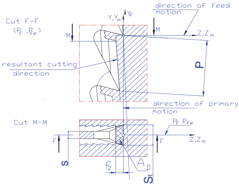
Fig. 2 Sawing kinematics on the sash gang saw and band sawing machine: f_z feed per tooth, s saw blade thickness, A_D area of the cut, P pitch, Y , Z and Y_M , Z_M machine coordinate and setting axes, Y_f f -set coordinate axis, P_{fe} working plane
