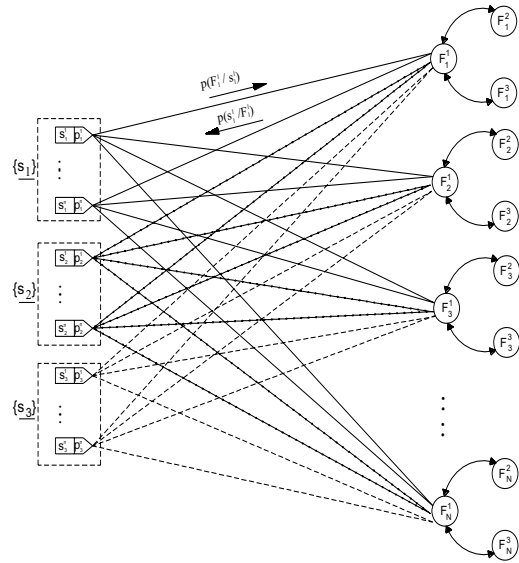
Fig.3. Topological diagnostic model of measurement circuits, where: F_1^1, F_2^1, \dots, F_N^1 – signals emitted from piezoelectric measuring transducers about z_1 aptitude; F_1^2, F_2^2, \dots, F_N^2 – signals emitted from piezoelectric measuring transducers about z_2 aptitude; F_1^3, \dots, F_N^3 – signals emitted from piezoelectric measuring transducers about z_3 aptitude; \{s_1\} state of full aptitude of a main subassembly of engine crankshaft piston assembly; \{s_2\} – state of partial aptitude; \{s_3\} – state of inaptitude; p(F_1^1 / s_1) – probability that emitted signal F_1^1 is observed on the condition that state s_1 occurs; p(s_1 / F_1^1) – probability that state s_1 occurs on the condition that emitted signal F_1^1 is observed.
