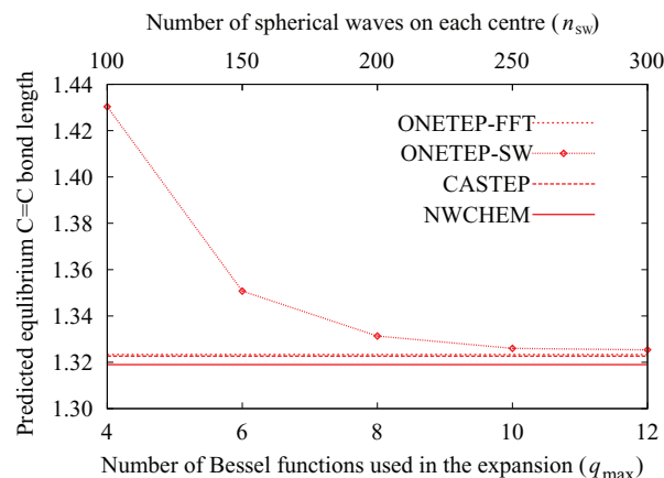
FIG. 14. Convergence of the predicted equilibrium C=C bondlength in ethene with the increasing quality of the auxiliary basis set. Calculations were performed with the Hartree-Fock approach. Spherical waves up to l_{\max} = 4 were used in the expansion. The total number of spherical waves used in the expansion, N_{\text{SW}} , is twice the value shown on the upper x axis, as two-centre expansion was performed.
