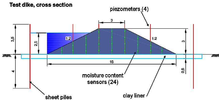
Fig. 2. The cross-section of the experimental dike in Poland with sensors placement
