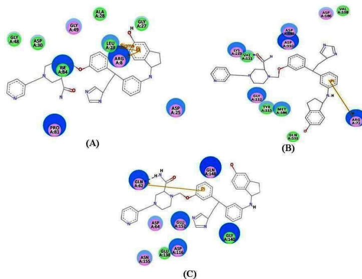
Fig. 3. Interaction analysis obtained for COM5 with HIV-1 enzymes from CDOCKER (flexible docking) approach. (A) COM5 interactions with HIV-1 protease; (B) COM5 interactions with HIV-1 reverse transcriptase; (C) COM5 interactions with HIV-1 integrase. (Color scheme: (A), (B) and (C), carbon atoms are represented in gray color, oxygen atoms in red and hydrogen atoms in white.)
