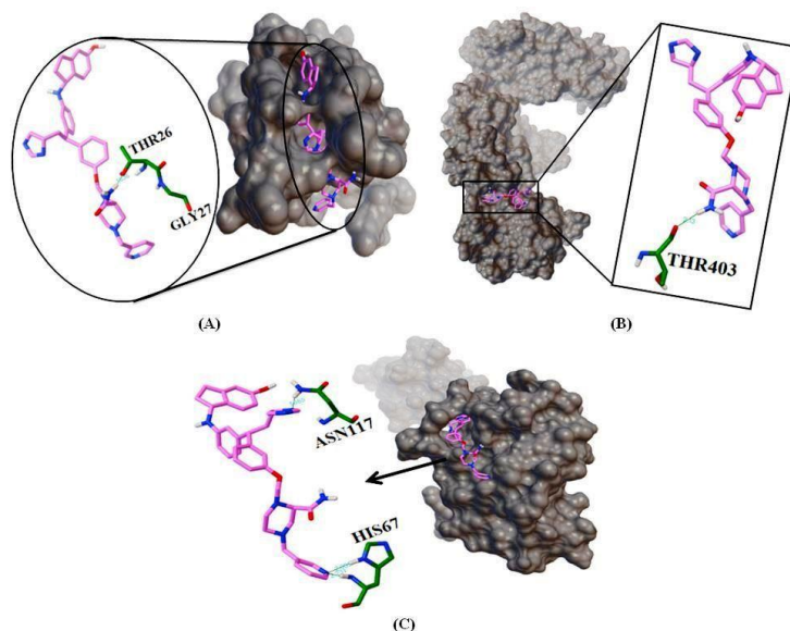
Fig. 4. Interactions obtained of COM5 with HIV-1 enzymes from AutoDock (rigid docking) approach. (A) COM5 interactions with HIV-1 protease; (B) COM5 interactions with HIV-1 reverse transcriptase; (C) COM5
