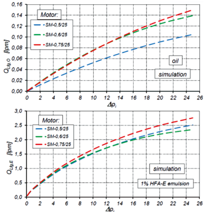
Fig. 9. Characteristics of oil and emulsion leakage flows in flat motor gaps (result of calculations)
