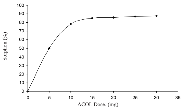
Fig. 7. CV adsorption as a function of AC of Oak leaves amounts (25 ml of 40 mg/l of CV, temp. 25°C and pH 7.0, shaking rate 130 rpm, contact time of 20 min.).
