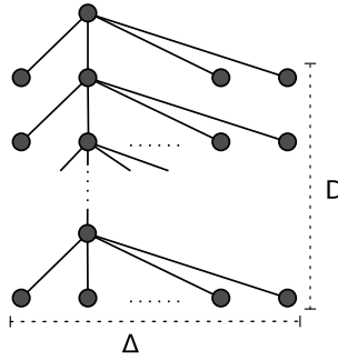
Fig. 3. An example of a tree in \mathcal{T}_{n,D} .
