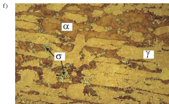
Fig.1. Microstructure of 2205 duplex steel after ageing : in 500°C temperature for e) 60 min., f) 600 min.
