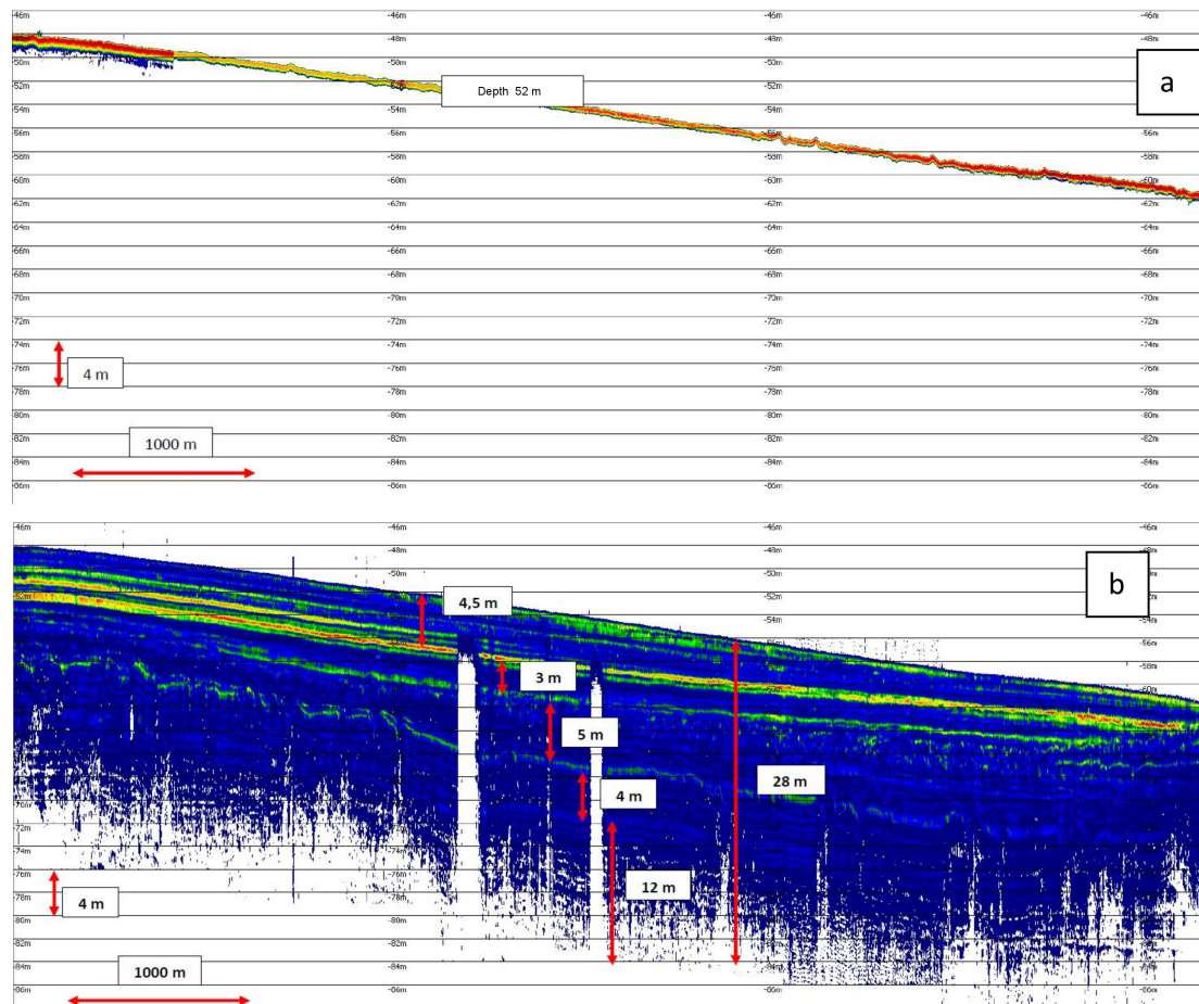
Fig. 6. Image of bottom taken in the Gulf of Gdansk using parametric echosounder; a) primary wave f = 100 kHz, b) difference frequency wave f = 5 kHz.
