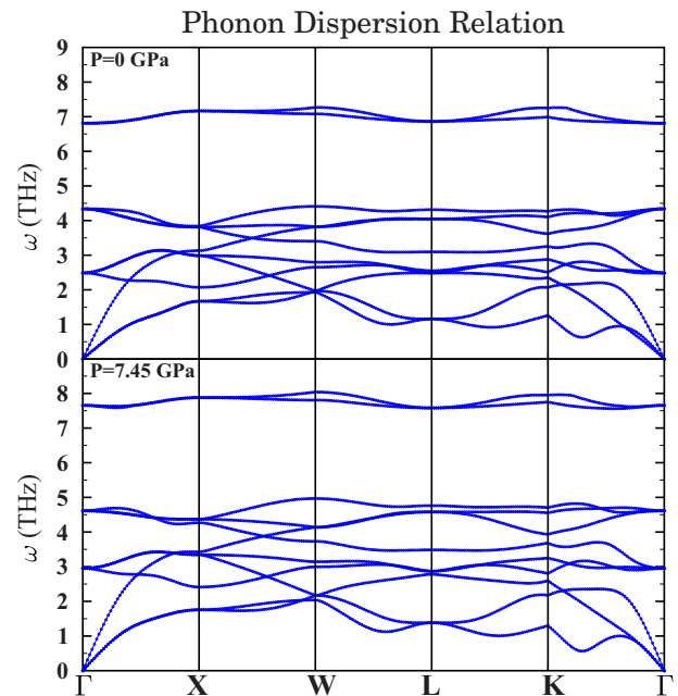
FIG. 9. (Color online) Phonon dispersion relations for HfPd 2 Al at 0 (top panel) and 7.45 GPa (bottom panel).
