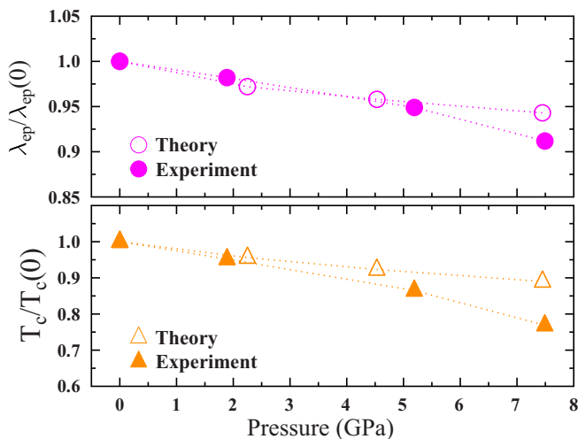
FIG. 10. (Color online) Relative changes of electron-phonon coupling parameter \lambda_{\text{ep}} (top panel) and critical temperature T_c (bottom panel) obtained from calculations (empty symbols) and measurements (full symbols). The overall trends are very similar, but theoretical results underestimate the experimentally observed changes for the highest pressures.
