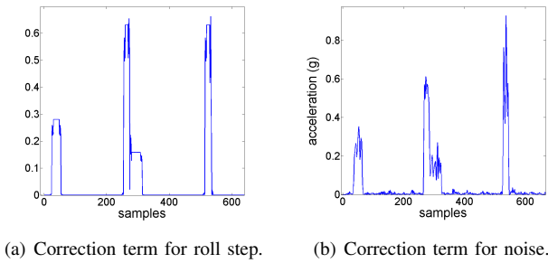
Fig. 6. Rotation dynamics (correction terms) for roll step.
