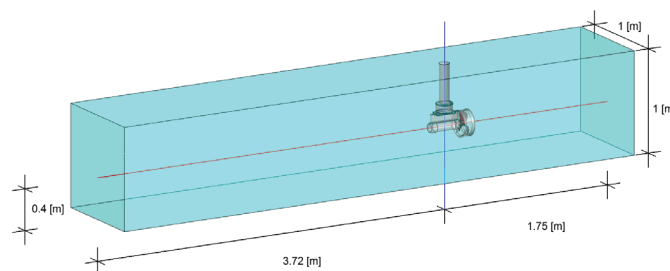
Fig. 7. Geometric parameters of CFD model No. 3
