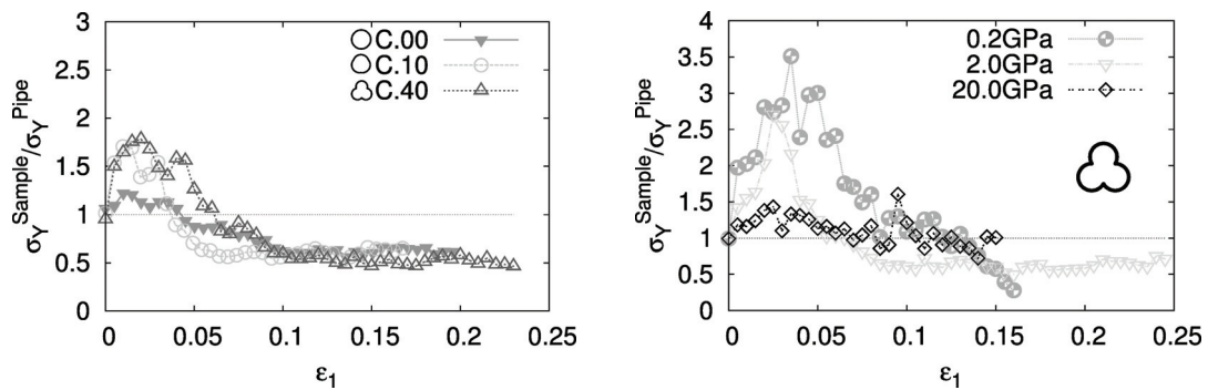
(a) Influence of particle shape, E = 2 \text{ GPa} , \mu^{\text{pipe}} = 0.0 ;
