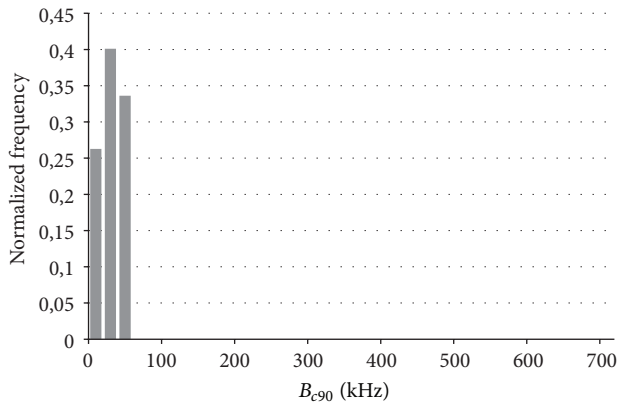
FIGURE 13: Histogram of coherence bandwidth values estimated from rms delay spread for correlation level 0.9 in the Gdansk city area.
