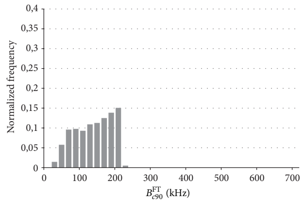
FIGURE 14: Histogram of coherence bandwidth values estimated from Fourier transform of PDP for correlation level 0.9 in the Gdansk city area.
