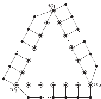
Figure 6: Graph G^k
