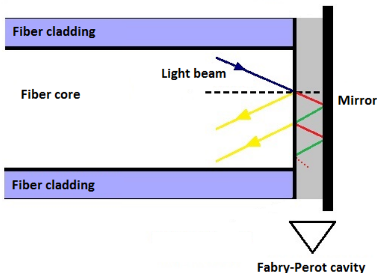
Figure 1. Fiber optic configuration of Fabry-Perot interferometer working at reflectance mode.
