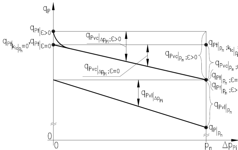
Fig.2 Subdivision of intensity of volumetric losses q_{p_i} = q_{Pvl} + q_{Pvc} per one shaft revolution in the pump working chambers, the losses dependent on indicated increase \Delta p_{pi} of pressure in the chambers, into intensity q_{Pvl}|\Delta p_{pi} of volumetric losses due to leakage (independent of liquid aeration coefficient \epsilon ) and intensity q_{Pvc}|\Delta p_{pi} of volumetric losses due to liquid compressibility, the subdivision made at pump capacity coefficient b_p = 1 :
