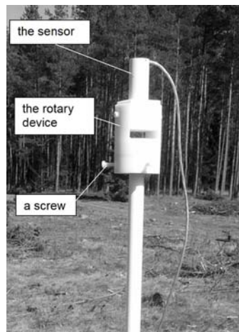
Fig. 8. Measuring workstation.
