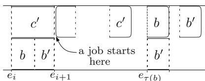
Fig. 4 The proof of Lemma 7: the positioning of jobs b, b' and c'
