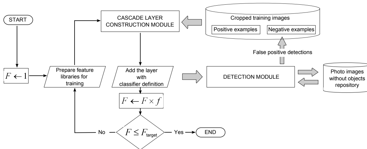
Fig. 4. The AdaBoost cascade training scheme.
