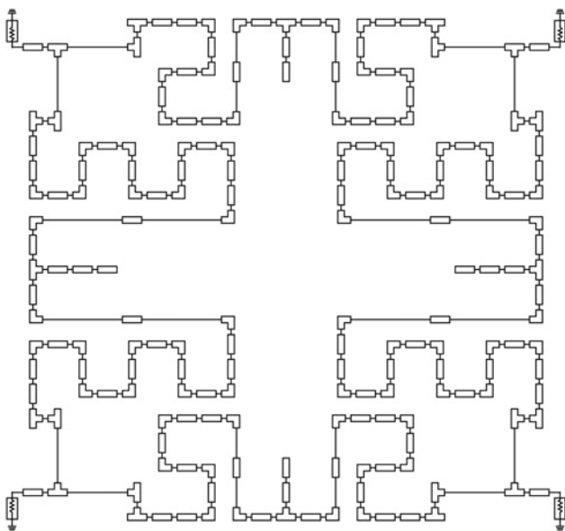
Fig. 7 Equivalent circuit ADS implementation ( R_{\text{circuit}} ) of the compact BLC from design case II
