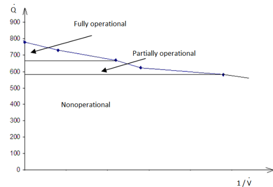
Fig.6. Three-level evaluation of the diesel oil cooler technical condition
