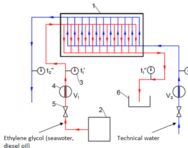
Fig. 2. Schematic diagram of the measurement stand : 1 – Plate heat exchanger, APV type U 121R, 2 – Small-capacity ultrathermostat, type UTM ZN-69 / CZSP - D3- 275, operates in the medium temperature range from -60 °C to 200°C, heater measurement uncertainty is \pm 0.03 °C, 3 – UT50 digital temperature meter, measurable temperature range from -40°C to 1000°C, measurement accuracy \pm (1 \div 3)\% , 4 - JS 16 Smart+ water meter, admissible measurement error within the (1 \div 3)\% range for the medium flow rates occurring during the tests, 5 – flow rate adjustment valve, 6 – overflow vessel
