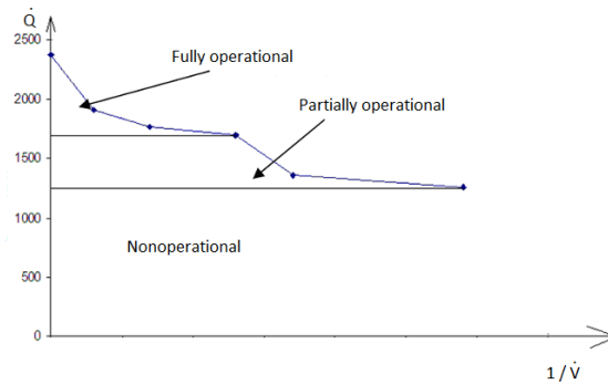
Fig.5. Three-level evaluation of the technical water cooler technical condition
