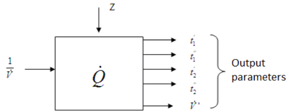
Fig.1. Schematic diagram of the diagnostic model of plate heat exchanger operation: 1/\dot{V} - inverse of the tested medium flow rate; \dot{Q} - thermal flux as a diagnostic parameter (state parameter), \dot{V}' - technical water flow rate, t'_1, t''_1 - cooled medium input and output temperatures, t'_2, t''_2 - cooling medium input and output temperatures, Z - disturbances (e.g. thermal losses to the environment, losses in the conduits)
