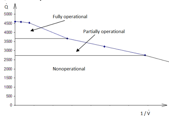
Fig.4. Three-level evaluation of the ethylene glycol cooler technical condition
