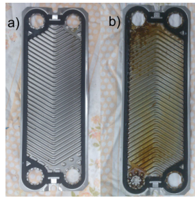
Fig. 3. Heat exchanger plates [5,6,7]: a) in fully operational condition, b) in partially operational condition
