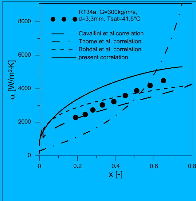
Fig. 16. Flow condensation heat transfer coefficient for R134a, Bohdal [9], d=3.3\text{ mm} .
