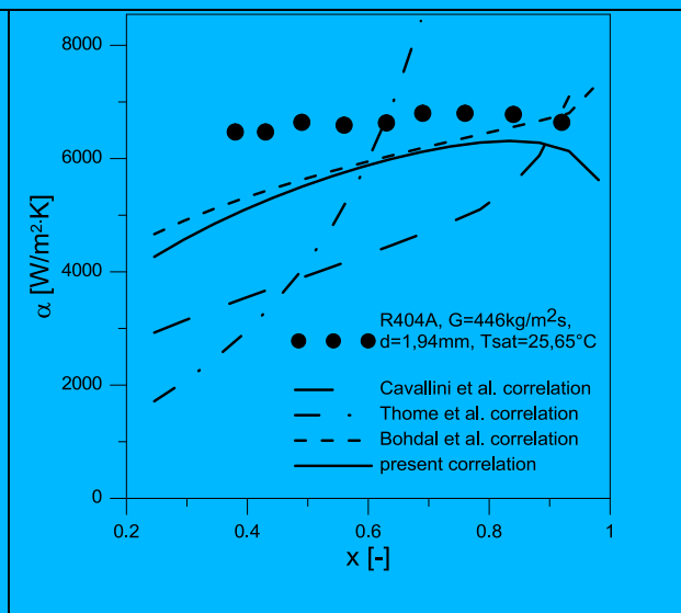
Fig. 19. Flow condensation heat transfer coefficient for R404A, Bohdal [9], d=1.94\text{mm} .
