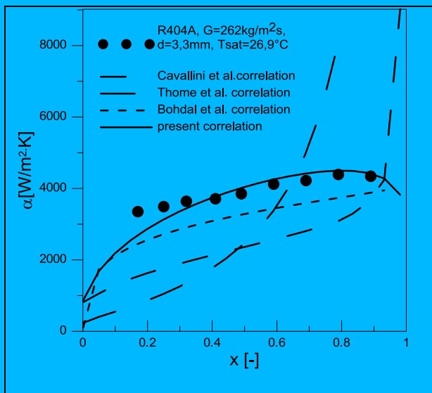
Fig. 18. Flow condensation heat transfer coefficient for R404A, Bohdal [9], d=3.3\text{m} .
