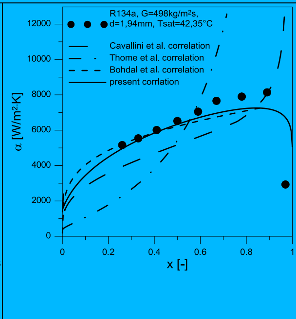
Fig. 17. Flow condensation heat transfer coefficient for R134a, Bohdal [9], d=1.94\text{mm} .
