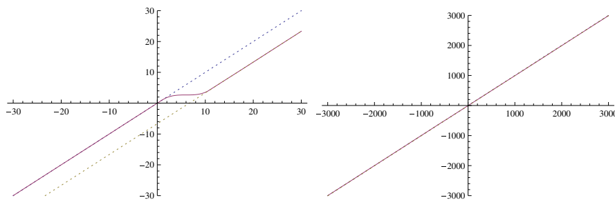
Fig. 1 Diophantine correspondence principle. Left f(x) that interpolates between f(x) = x (for x \leq 1 ) and f(x) = x - 20/3 (for x \geq 10 ). In the transition region f(x) = (-16 + 108x - 18x^2 + x^3)/75 . f : \mathbb{R} \rightarrow \mathbb{R} is bijective and satisfies f(0) = 0, f(1) = 1 . Arithmetic defined in terms of f is non-Diophantine, but is well approximated by the standard Diophantine case f(x) = x if x is large enough. Right the same f(x) but plotted in a different scale. Here, f(x) is practically indistinguishable from f(x) = x and thus the resulting arithmetic is effectively Diophantine
