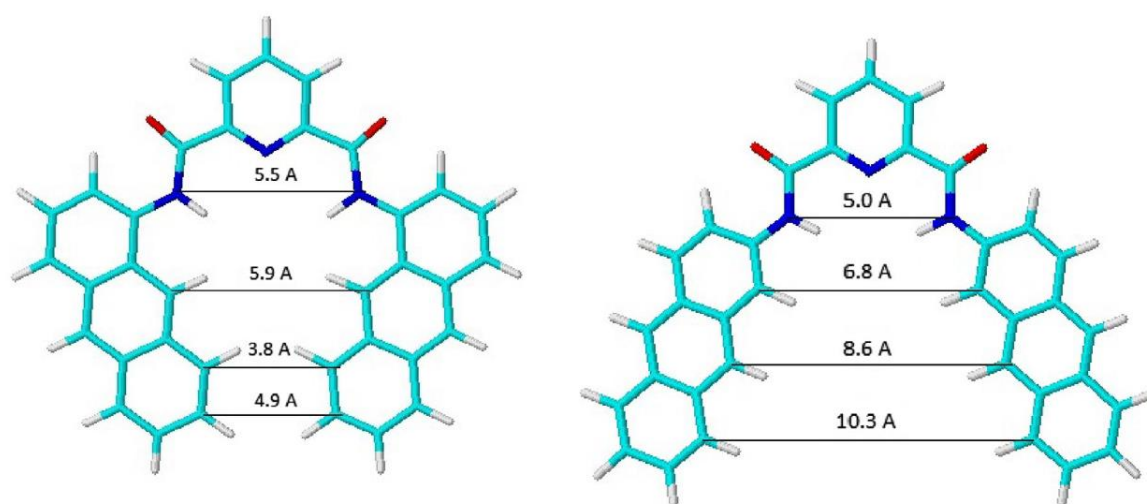
Figure 7. Optimised structures (AM1) of 'free' ligands 3 and 4 showing size of molecular pseudo-cavity as a distance of N-N and C-C atoms.
