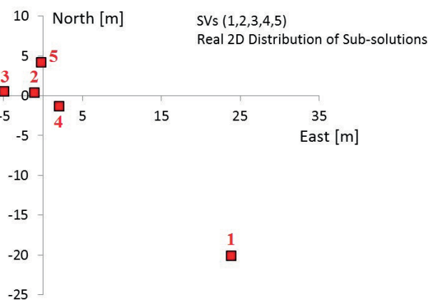
Fig. 7. Distribution of sub-solutions for drawn values of pseudorange measurements random errors. Red squares marked shift of sub-solutions related to the positioning solution. Numbers at squares indicate number of satellite excluded from the positioning solution
