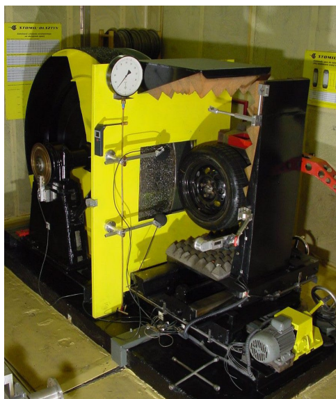
Figure 1. Roadwheel facility at TUG with external drum of 1.7 m diameter.
