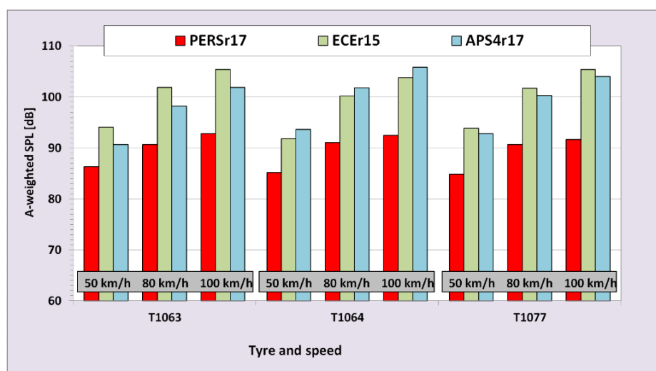
Figure 1. A-weighted sound pressure level (SPL) for passenger car tire.
