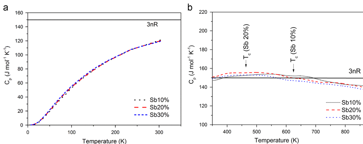
Fig. 1. Temperature dependence of heat capacity of \text{LaNb}_{0.9}\text{Sb}_{0.1}\text{O}_4 , \text{LaNb}_{0.8}\text{Sb}_{0.2}\text{O}_4 and \text{LaNb}_{0.7}\text{Sb}_{0.3}\text{O}_4 samples in low (a) and high (b) temperature ranges. T_c (Sb 10%) and T_c (Sb 20%) are temperatures of the scheelite–fergusonite phase transition of \text{LaNb}_{0.9}\text{Sb}_{0.1}\text{O}_4 , \text{LaNb}_{0.8}\text{Sb}_{0.2}\text{O}_4 respectively.
