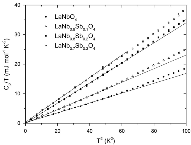
Fig. 2. The heat capacity divided by temperature plotted as a function of T^2 . Solid lines correspond to the low temperature fitting by Eq. (1).
