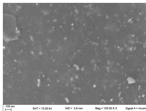
Figure 2. SEM image of the Fe-FAG powder displaying nanometric spherules (possibly agglomerates of metallic Fe or carbon-iron compounds).
