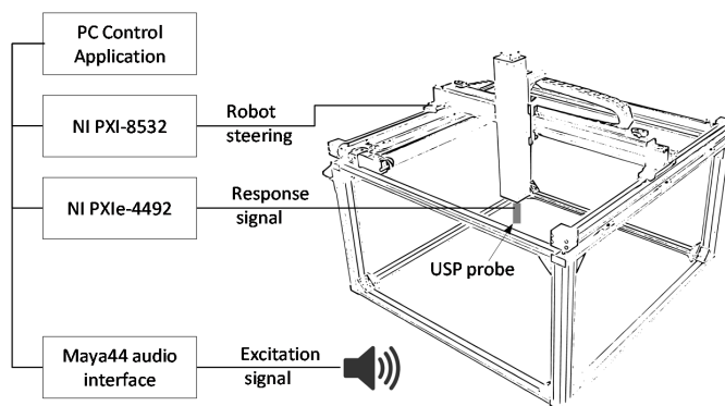
Fig. 1. A diagram of the measurement system.
