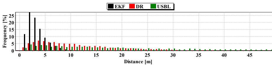
Figure 26. Histogram of the reference position distance from the position estimated by EKF and DR methods and determined by the USBL system (one hundred passages).
