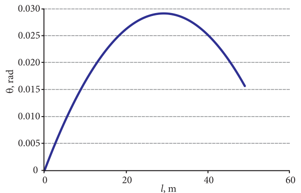
Fig. 2. Slope of the tangent \theta(l) chart, described by formula (13), for S-shaped joining of circular arcs with curvatures k_1 = \frac{1}{500} rad/m and k_2 = -\frac{1}{700} rad/m ( l_k = 50 m)
