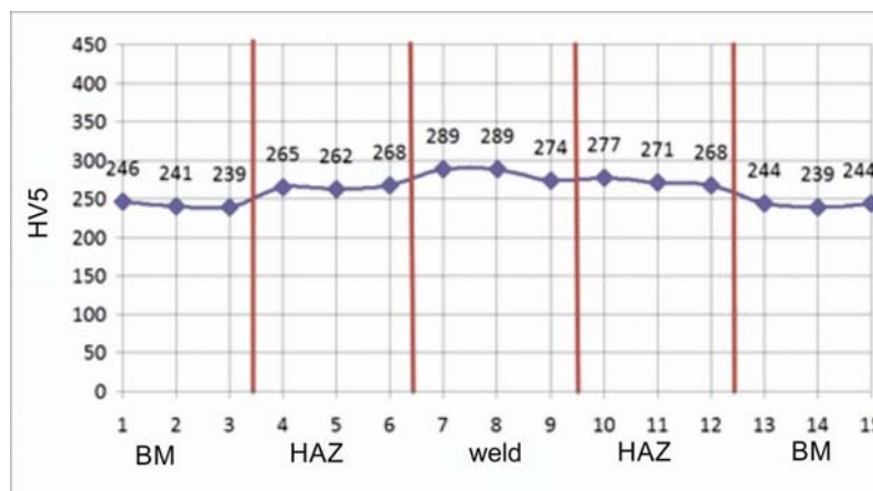
Fig. 12. Hardness distribution on joint cross section performed under water (W4) with heat input 3.0 kJ/mm
