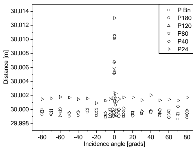
Figure 15: Measured distance to light blue plates of varying roughness, depending on the incidence angle of the laser beam (measurement uncertainty – 3 mm)
