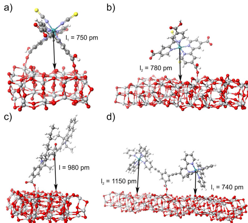
Figure 3. Possible binding schemes of (a,b) N719, (c) SQ2, (d) B1 to surface of anatase \text{TiO}_2 cluster with indicated distance between the \text{TiO}_2 surface and a central atom (a,b,d) or a geometrical center of hole localized on a dye molecule (c).
