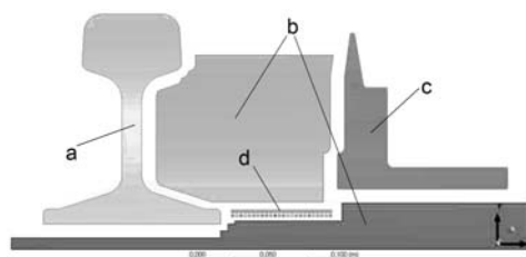
Fig. 2. The model of the railway turnout with the induction heater (a - a fixed rail, b - an 'ice', c - a moveable rail, d - the induction heater)
