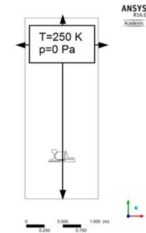
Fig. 4 The model of the railway turnout with the induction resistance heater
