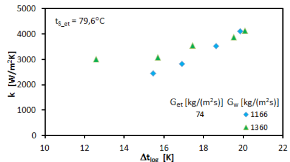
Figure 9. Overall heat transfer coefficient versus the logarithmic mean temperature difference.
