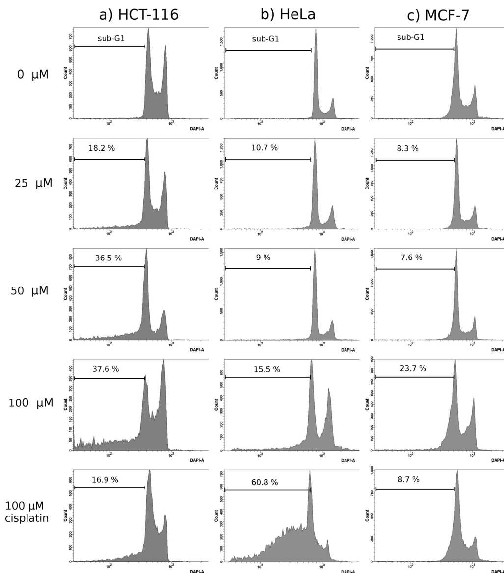
Figure 4. HCT-116, HeLa and MCF-7 cell cycle 24 h induction with 1,2,4-triazine derivatives (representative results). HCT-116 (a); HeLa (b) treated with 37 (0–100 \mu\text{M} ) and cisplatin (100 \mu\text{M} ); MCF-7 (c) treated with 46 (0–100 \mu\text{M} ) and cisplatin (100 \mu\text{M} ).
