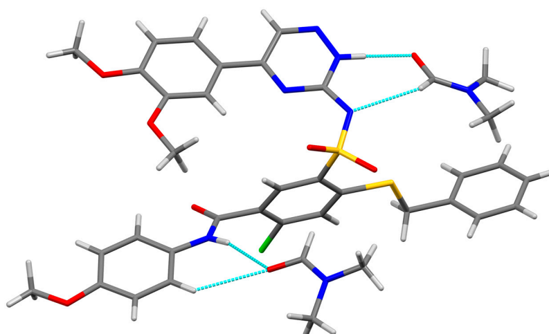
Figure 2. View of half of the independent unit (one sulfonamide and two DMF molecules) showing the general arrangement of atoms in 59 and N–H···O type hydrogen bonds.
